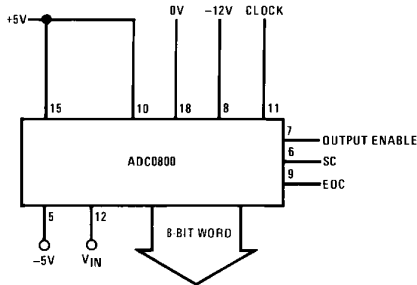
General Connection
